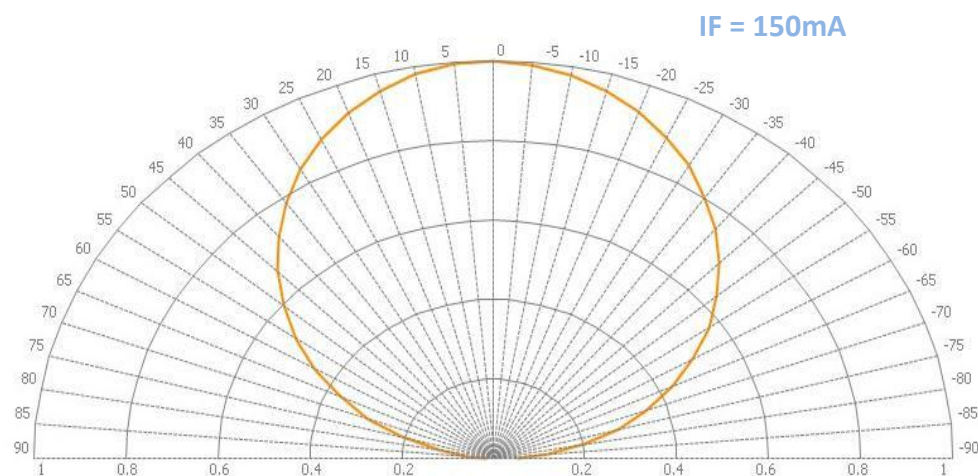
Fig 2. Viewing Angle Distribulon（发光角度）, Ta = 25℃, RH60%
