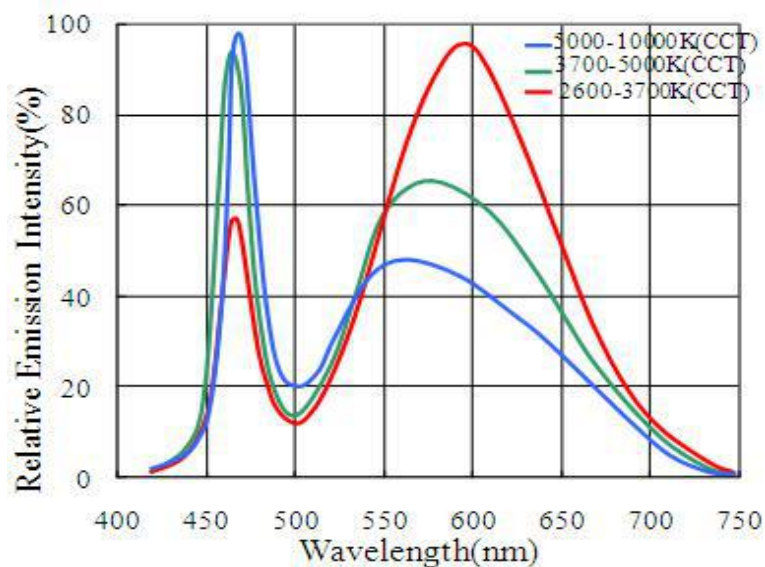
Fig 1. Color Spectrum（光谱图）, Ta = 25℃, RH60%
